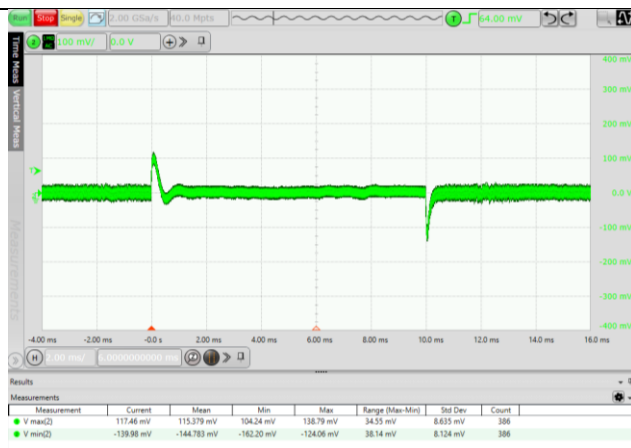
Fig. 5.7 25% -50% -25%IO Dynamic waveform (VIN=24V)
