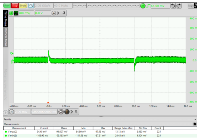
Fig. 5.6 Output voltage ripple waveform (VIN=24V, 100% Load)
