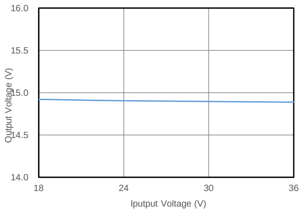
Fig. 5.3 Output Voltage vs. Input Voltage (100% Load)
