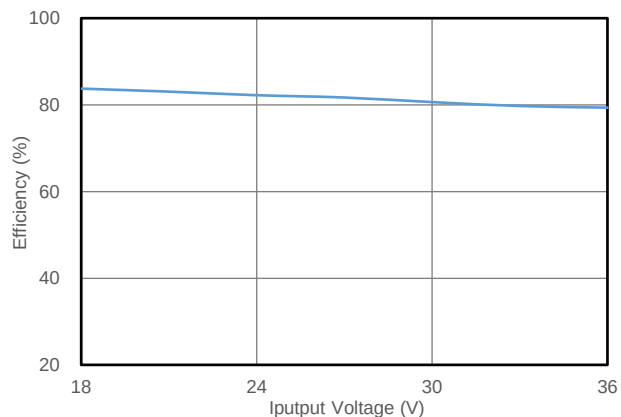
Fig. 5.4 Efficiency vs. Input Voltage (100% Load)
