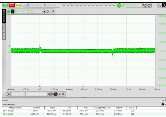
Fig. 5.6 Output voltage ripple waveform (VIN=24V, 100% Load)
