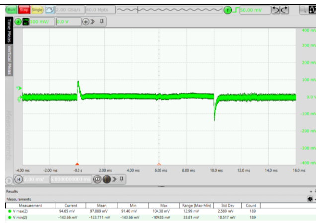
Fig. 5.5 Output voltage ripple waveform (VIN=24V, 5% Load)
