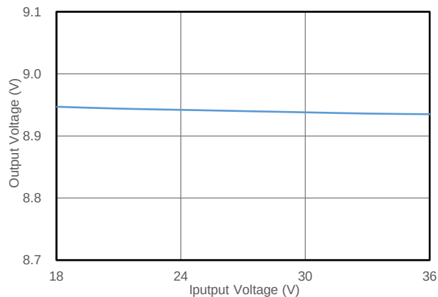
Fig. 5.3 Output Voltage vs. Input Voltage (100% Load)
