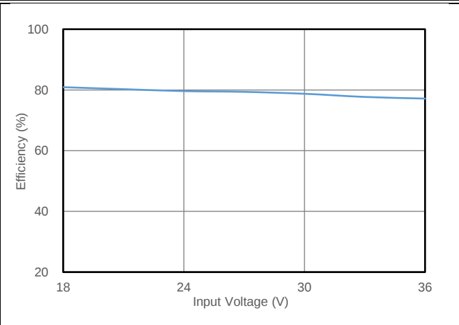
Fig. 5.4 Efficiency vs. Input Voltage (100% Load)
