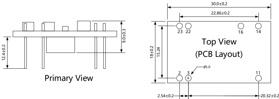
Fig. 3.3 Package Outline
