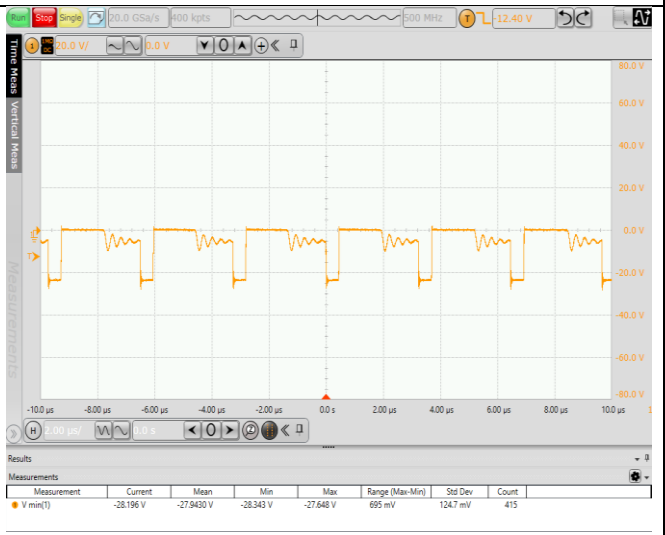
Fig. 5.10 Secondary-side output diode stress waveform (VIN=36V, 100% Load)
