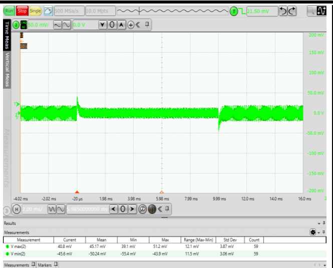
Fig. 5.8 50% -75% -50%IO Dynamic waveform (VIN=24V)
