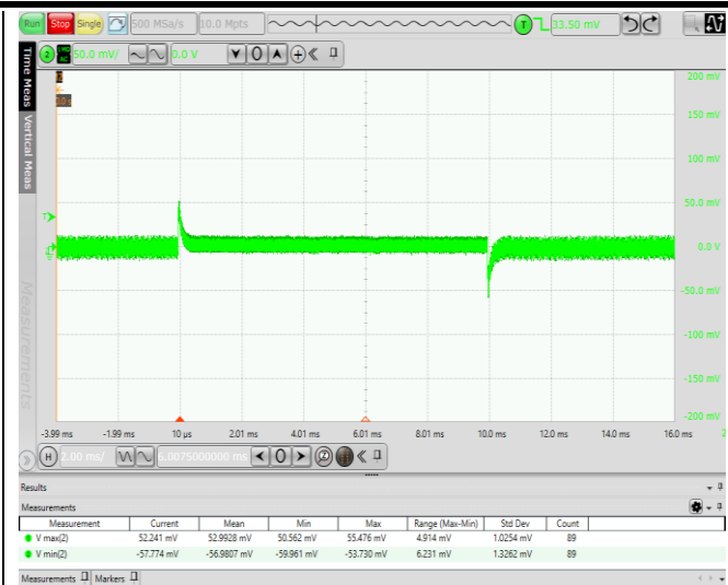
Fig. 5.7 25% -50% -25%IO Dynamic waveform (VIN=24V)
