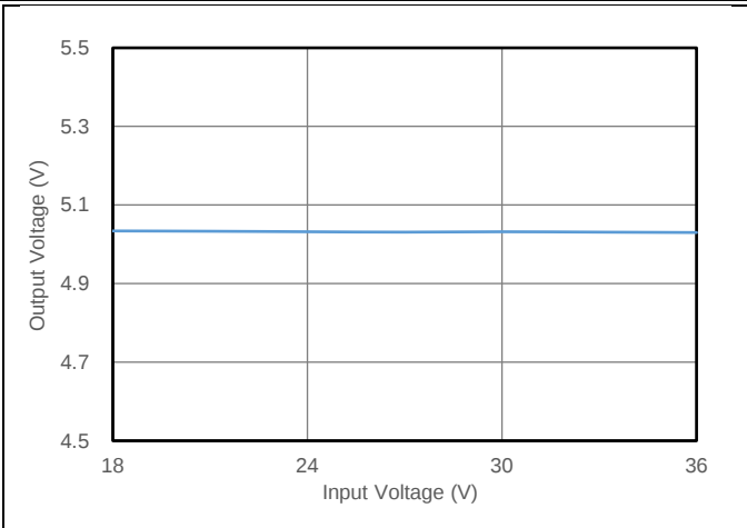
Fig. 5.3 Output Voltage vs. Input Voltage (100% Load)
