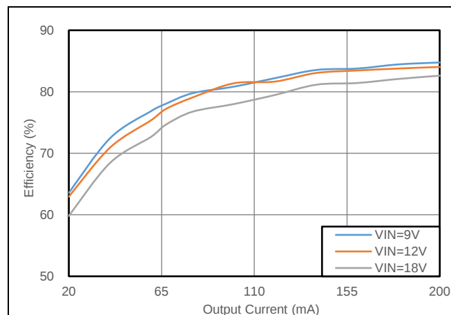
Fig. 5.1 Efficiency vs. Output Current
