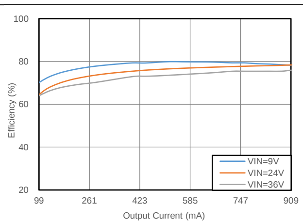
Fig. 5.2 Efficiency vs. Output Current
