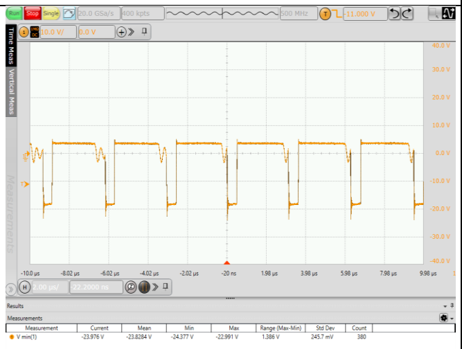
Fig. 5.8 50% -75% -50%IO Dynamic waveform (VIN=24V)
