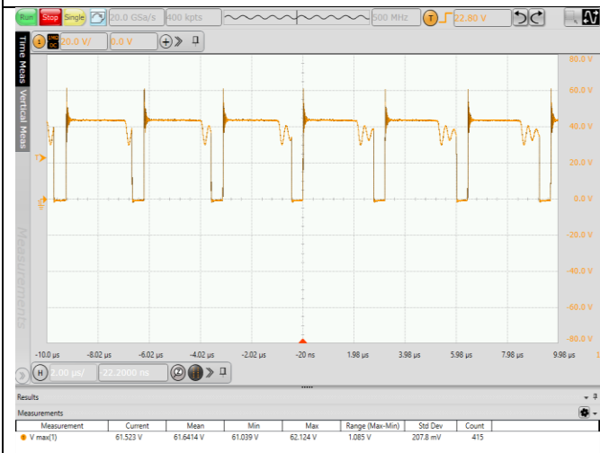
Fig. 5.7 25% -50% -25%IO Dynamic waveform (VIN=24V)
